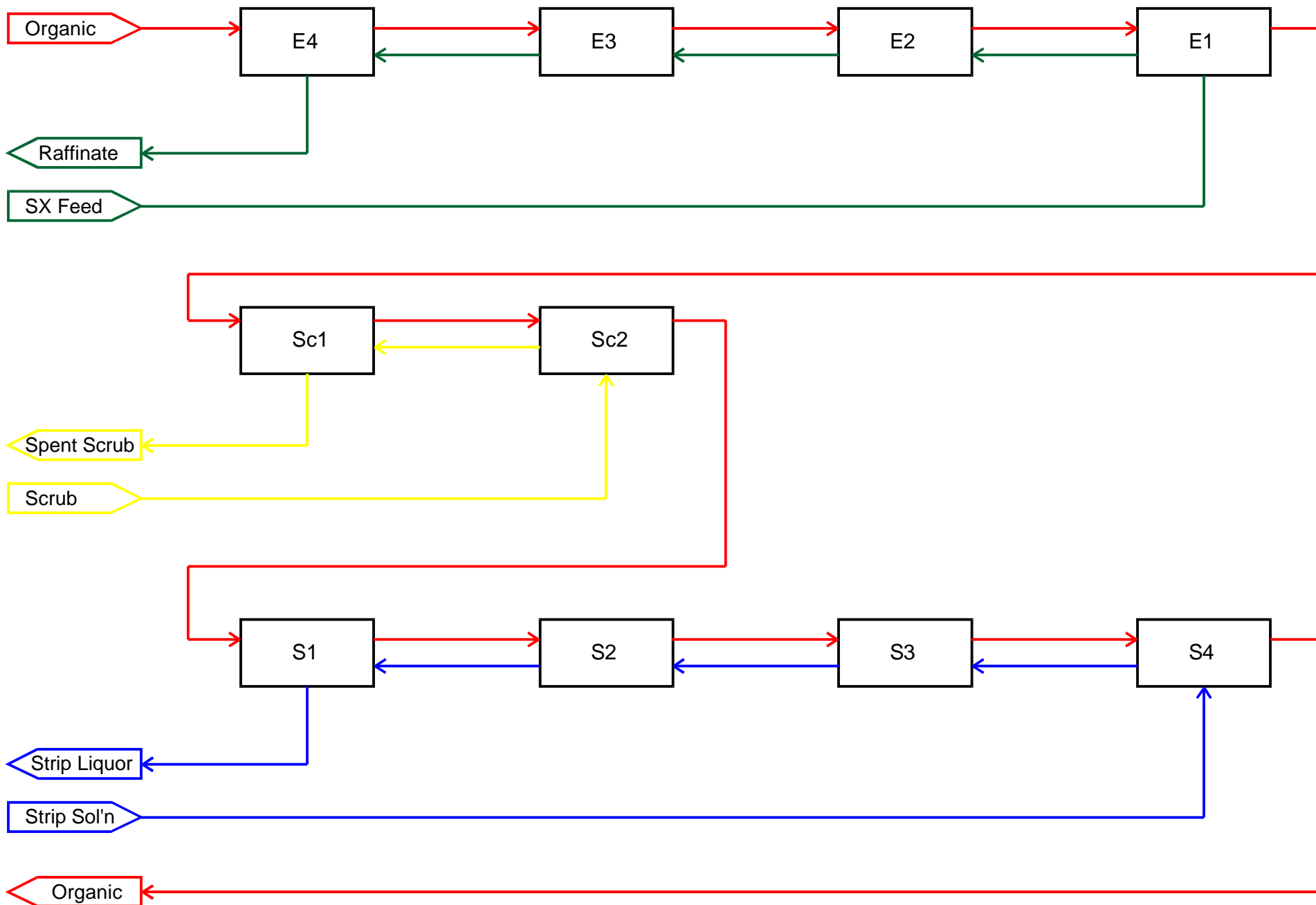
Flow diagram of a typical solvent extraction process.
